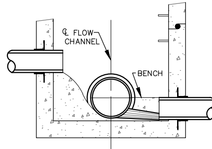
TYPICAL DETAIL 2' DROP OR LESS
