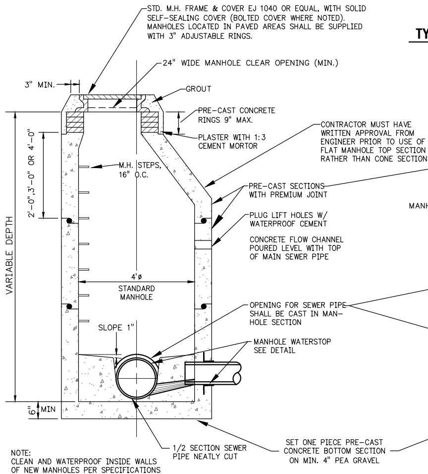
SECTION THRU STANDARD MANHOLE
