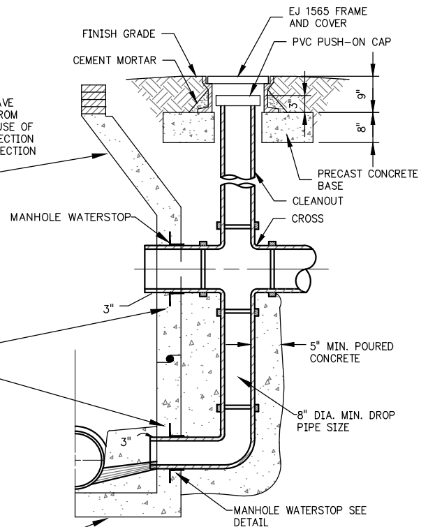
TYPICAL DETAIL 2' DROP OR LESS
